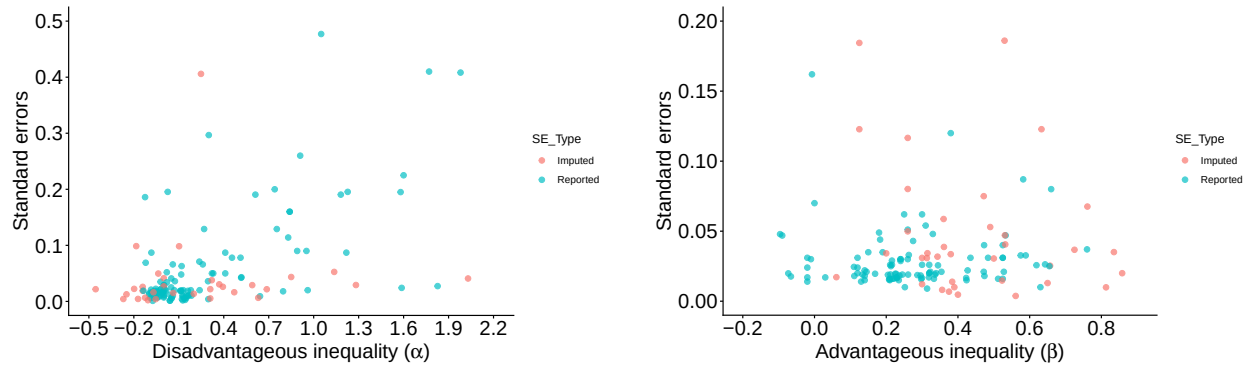
Figure K.3: Scatter Plots of \alpha and \beta SEs as a Function of SE Type. Note: The x-axis in the plot for \alpha is truncated at 2.2; the x-axis in the plot for \beta is truncated at -0.2 and 0.9 for better visual rendering.
