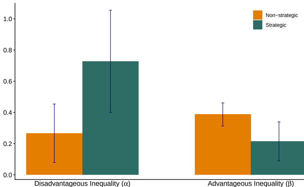
Figure 5: ML Estimates of Disadvantageous Inequality ( \alpha ) and Advantageous Inequality ( \beta ) in the Sub-Samples with Strategic vs Non Strategic Environments. Notes: Estimates are from columns 1 and 5 in Table 6; vertical bars are 95% confidence intervals.
