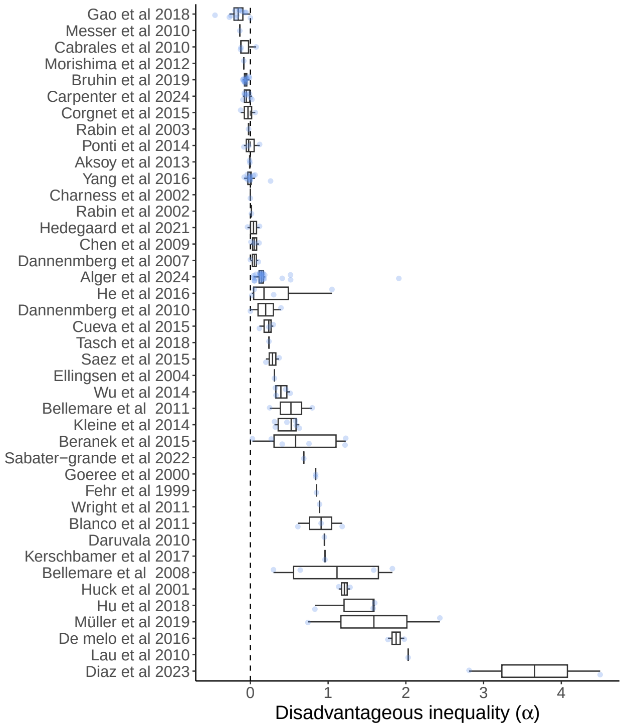
Figure J.1: Boxplots of sensitivity to disadvantageous inequality estimates ( \alpha ) by paper.
