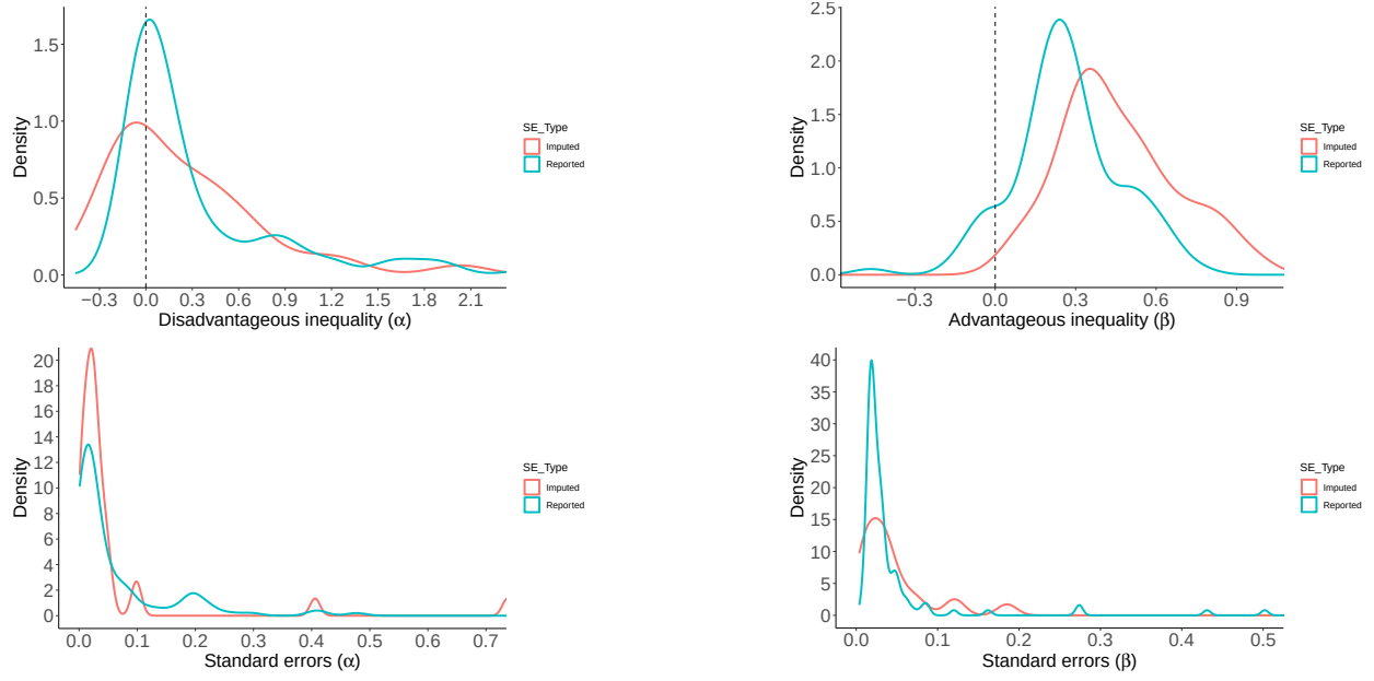
Figure K.2: Distribution of Estimates and SEs for \alpha and \beta as Function of SE Type. Note: The top two graphs show kernel density estimates (Gaussian with Silverman’s rule of thumb) for the subsets of parameters with reported vs. imputed SEs; the bottom two graphs show kernel density estimates of SEs in the two subgroups; the x-axis in the density plot for \alpha is truncated at 2.2; the x-axis in the density plot for \beta is truncated at -0.5 and 0.9 for better visual rendering but the kernel density uses all estimates in both cases.
