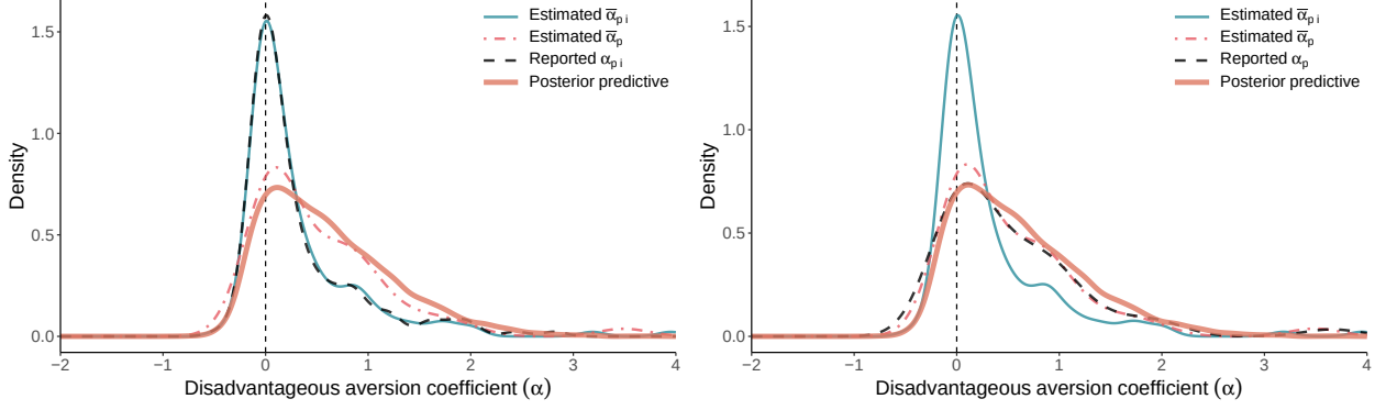
Figure D.3: Distribution of empirical, estimated and predictive distribution of the Disadvantageous Inequality Coefficient ( \alpha ). The left Figure plots all the reported estimates for \alpha in our dataset. The right Figure plots only one estimate per paper. In case the paper reports multiple estimate, we compute and consider only the mean.
